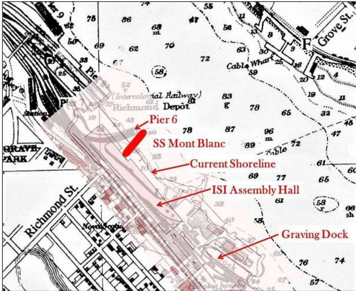
British Admiralty Halifax Chart 1416 (in black) showing the locations of Pier 6, SS Mont Blanc and SS Iro, overlaid with a scale site plan of the current Halifax Shipyard (in red), illustrating their relative positions
