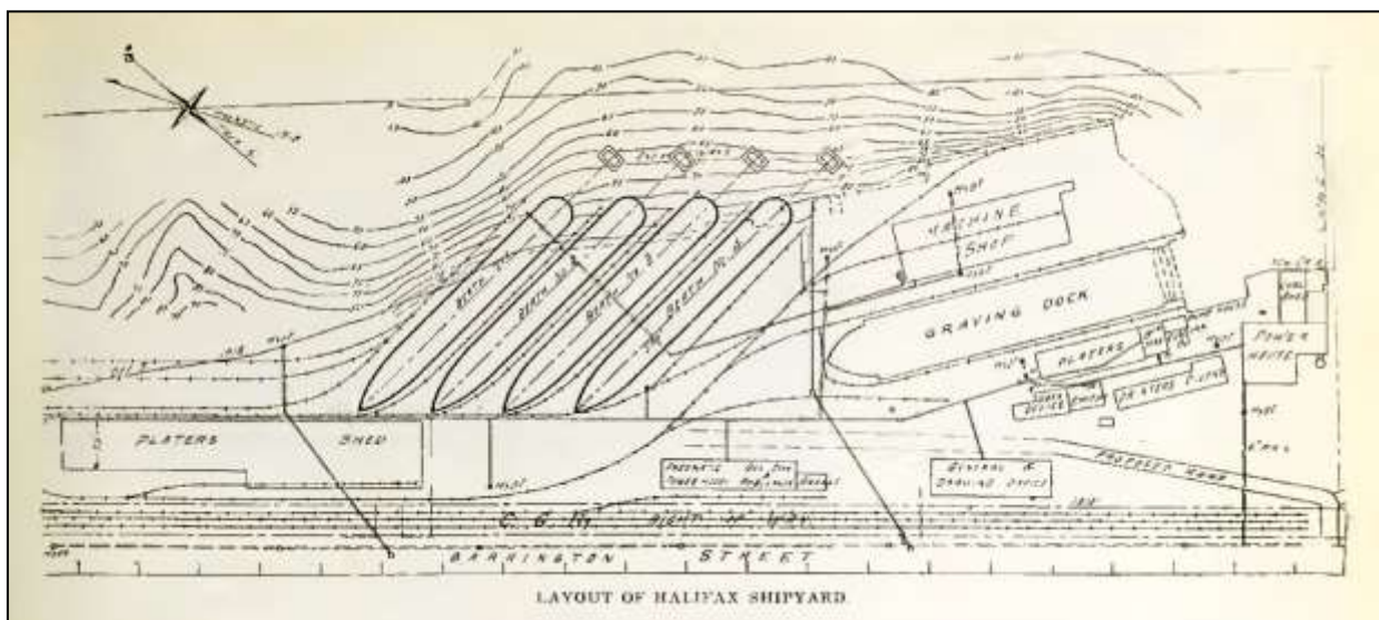
The planned layout of the Halifax Shipyards circa 1919 following the 1917 Halifax Explosion
